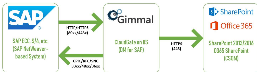
Figure 2-5 CSOM Deployment Model
